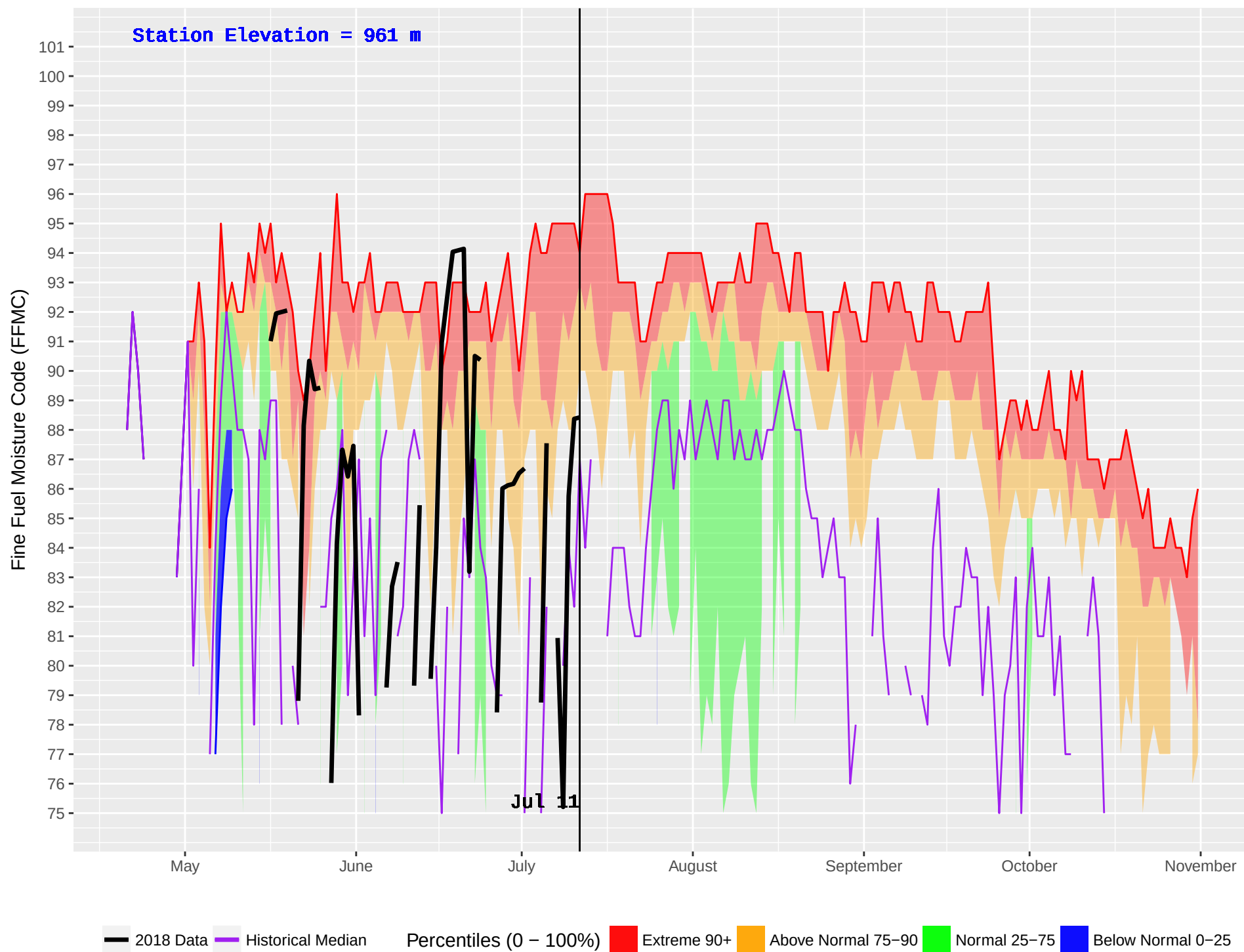
HOLY CROSS 2 (654) : Historical (1998–2016) and Current (2018) Noon Fine Fuel Moisture Code (FFMC)
