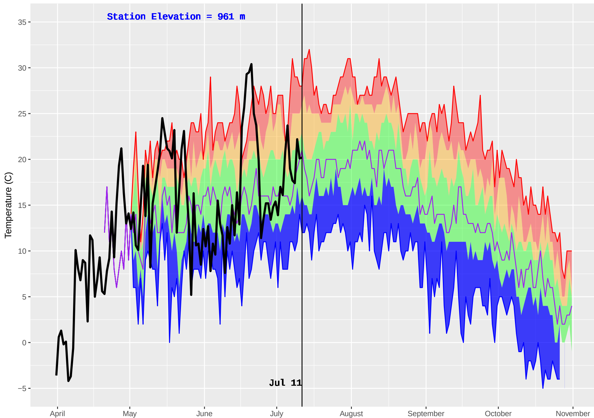
HOLY CROSS 2 (654) : Historical (1998–2016) and Current (2018) Noon Temperature
